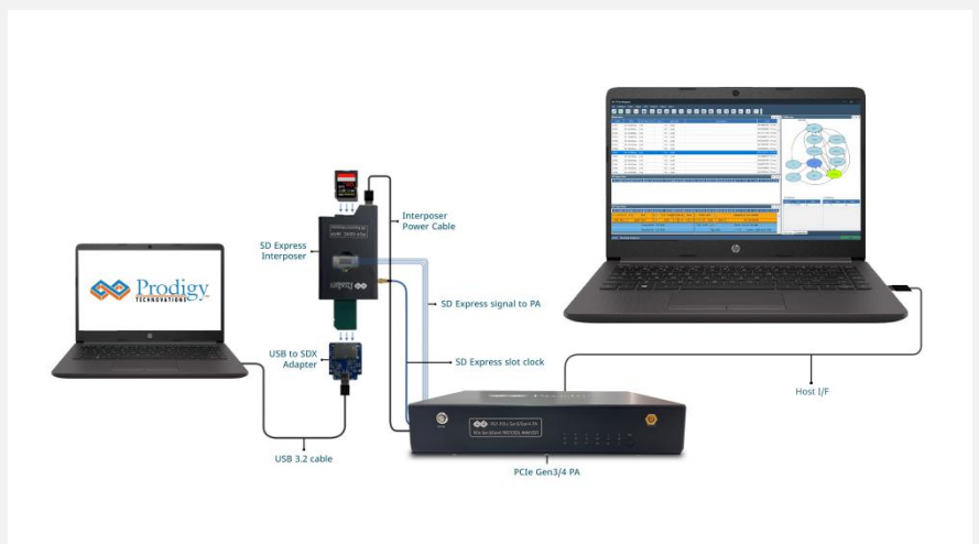
SD Express Interposer connection setup
