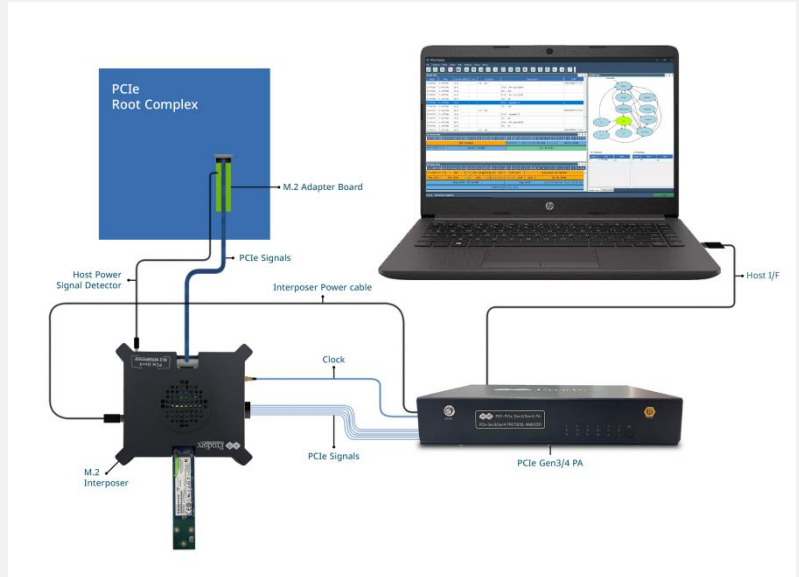
M.2 Interposer connection setup
